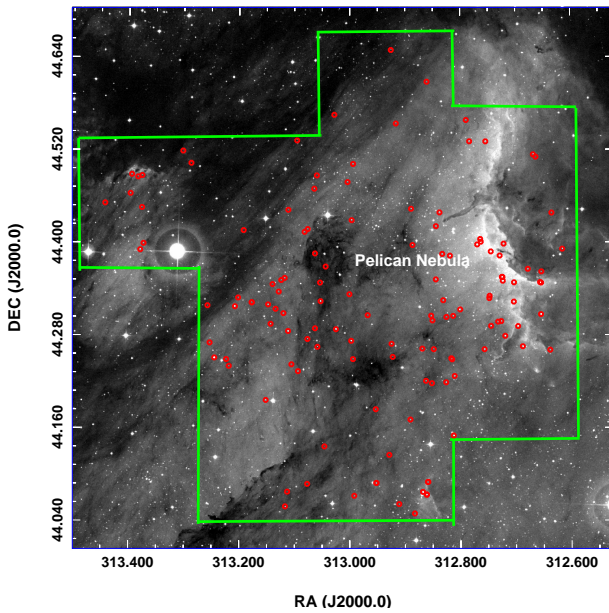
Figure 1. Left Panel: DSS2R image of the IC 5070 region. Area enclosed with the green polygon represents the coverage of the present survey of H \alpha emission-line stars with the HCT ( \sim 0.29 square degrees). The red circles represent emission-line stars identified in the present work. Right panel: Color-inverted slitless H \alpha image for one of the sub-regions. Stars with enhanced H \alpha emission are marked with the red circles.
