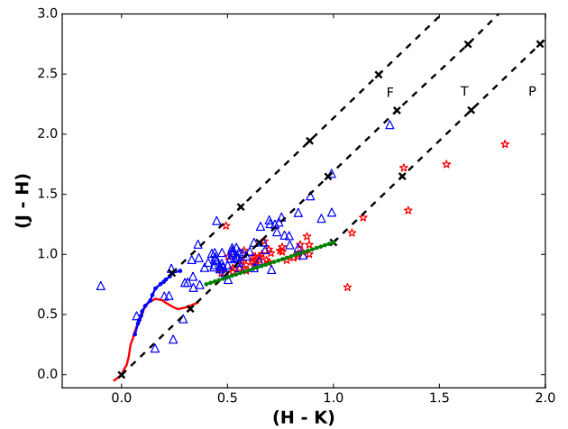
Figure 4. NIR color-color diagram for the emission-line stars in the IC 5070 region shown in Fig. 1. NIR counterparts of H\alpha emission stars taken from YSO catalog of Das et al. (2021) and 2MASS data are shown with star symbols and triangles, respectively. The thick red and blue curves represent the locus of the main-sequence (MS) stars and the giants, respectively (Bessell & Brett, 1988). The thin green line shows the CTTS locus (Meyer et al. , 1997). The three parallel black dashed lines drawn from the base of the MS locus, the turning point of the MS locus, and the tip of the CTTS locus are the reddening vectors.
