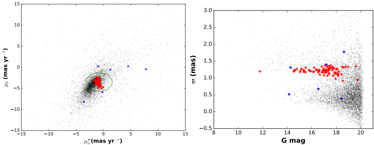
Figure 2. Vector point diagram (left panel) and parallax vs. magnitude (right panel) for the stars in the IC 5070 region. Black dots represent the sources within the region in Fig. 1 and red star symbols are the H\alpha emission line sources detected in the present survey. The green ellipse show the three- \sigma boundary around the mean proper motion values (see text).
